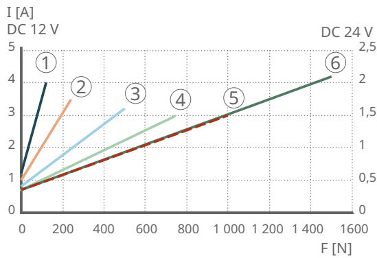
5 Strom-Last-Diagramm CAHB-10
