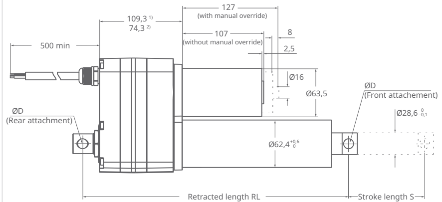
39 Side view dimensions for CAHB-21E, CAHB-21S
