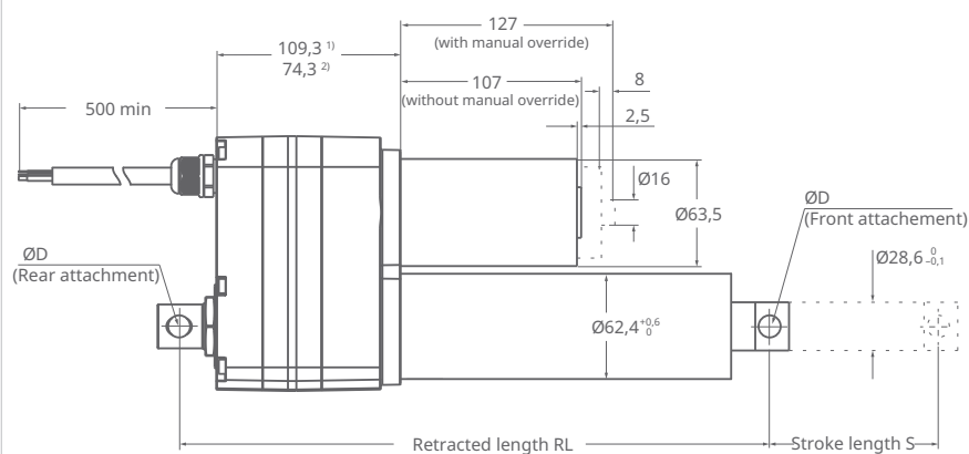
48 Side view dimensions for CAHB-22E, CAHB-22S
