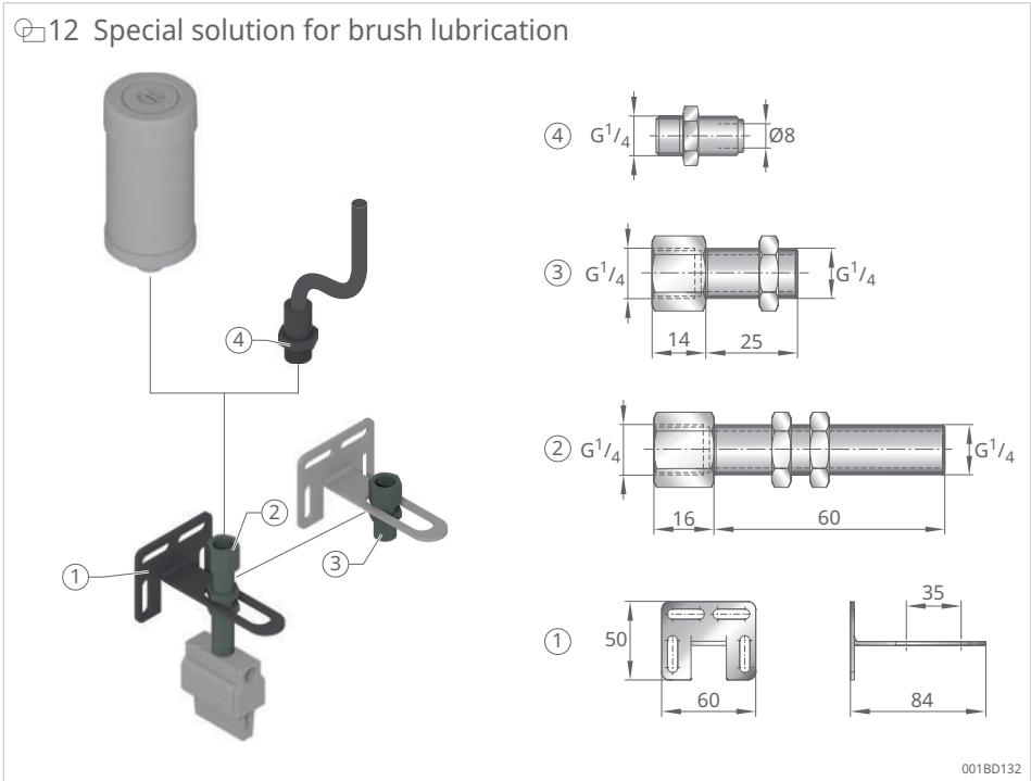
19 Ordering example: Special solution for brush lubrication
