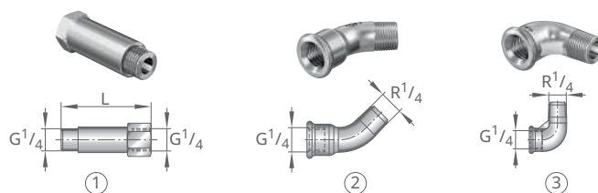
69 Screw-in connecting pieces: Product group H
