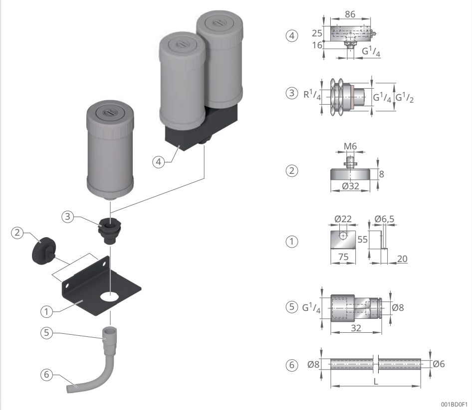
8 Mounting bracket with magnetic foot and optional twin adapter
