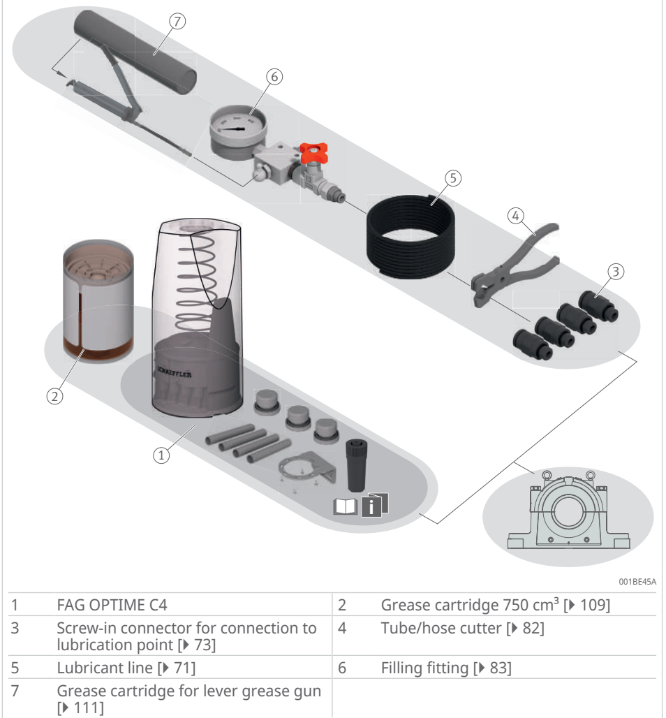
54 FAG OPTIME C4 with grease lubrication, DC 24 V
