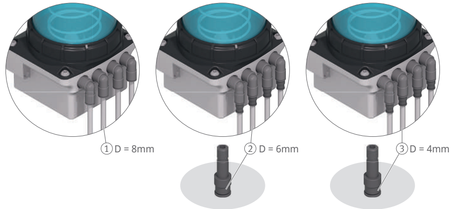
30 Connection adapter for direct connection to the outlet on the CONCEPT4
